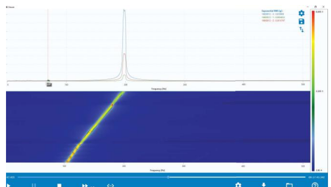
SPECTROGRAM FEATURE
